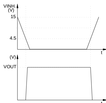
INHIBIT DIAGRAM
