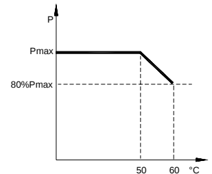
TEMP. DERATING
